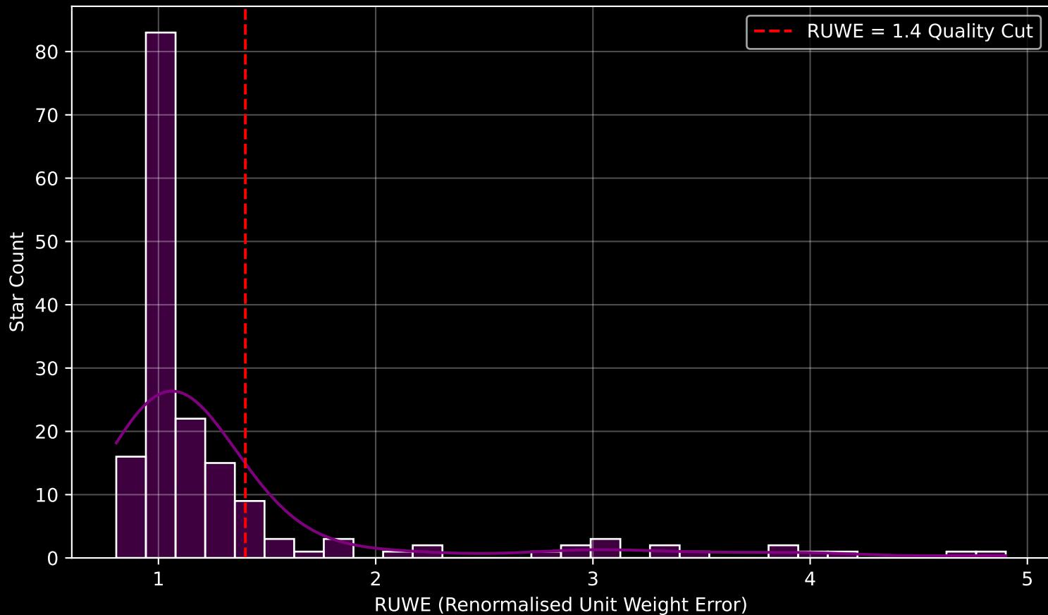
GAPOGEE DR17 Field [163+38_MGA] RUWE Distribution (n= 170)
