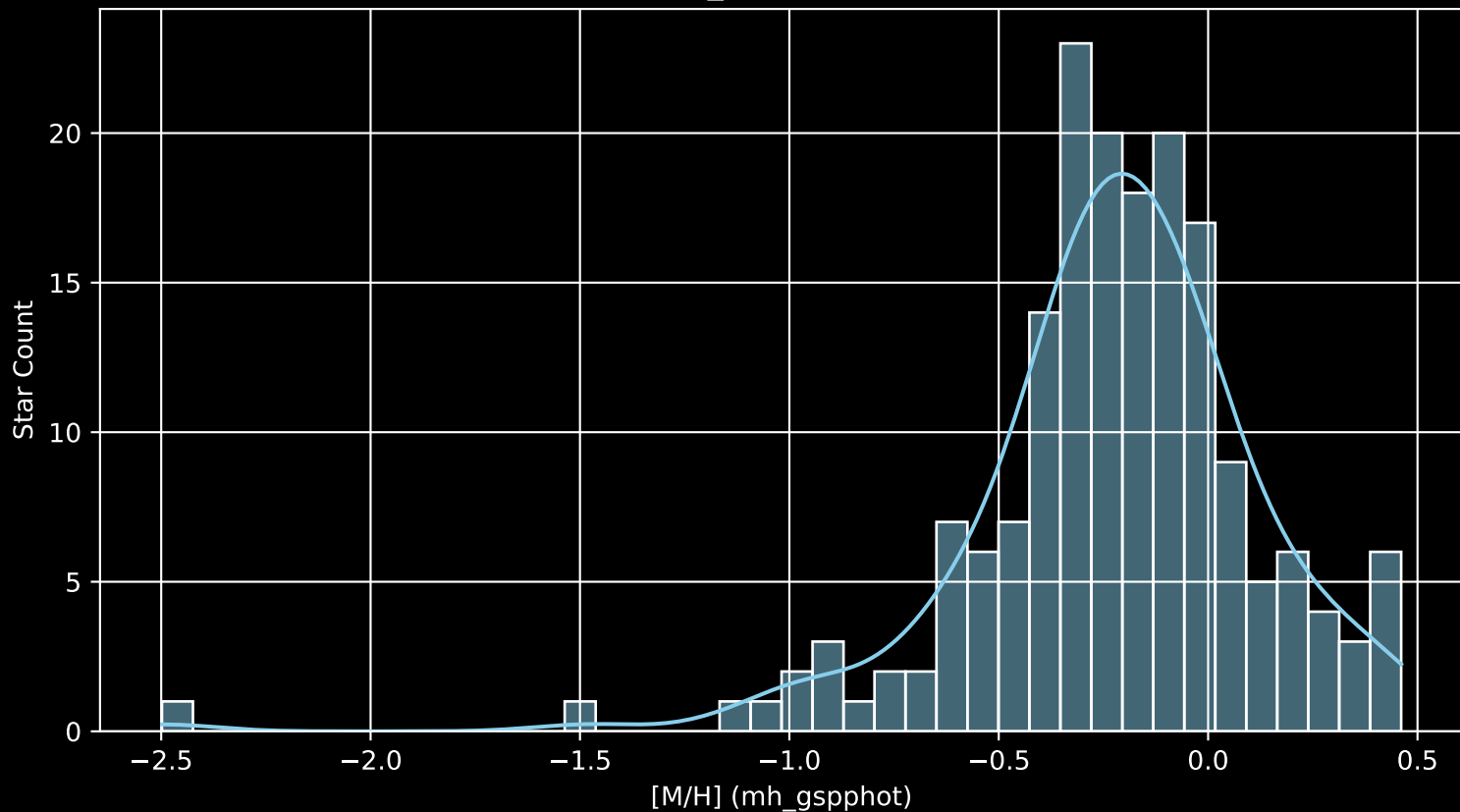
APOGEE DR17 Field: [163+38_MGA [M/H] (mh_gspphot) (n= 179)
