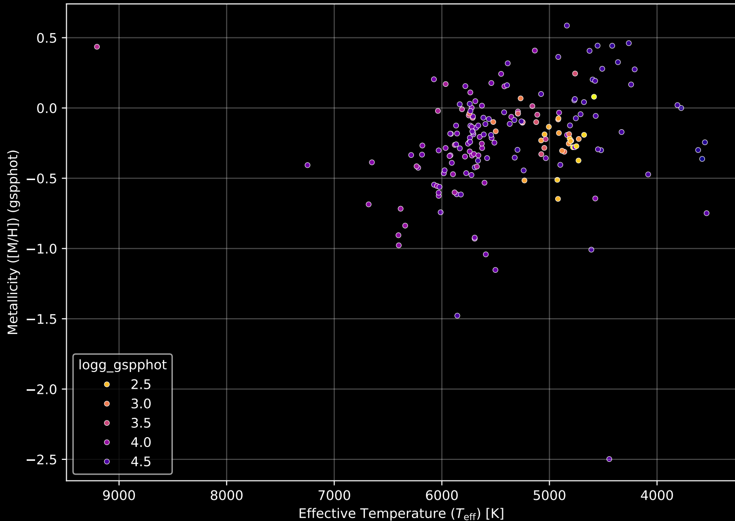
APOGEE DR17 Field: [163+38_MGA] Stellar Population Parameters (n= 180)
