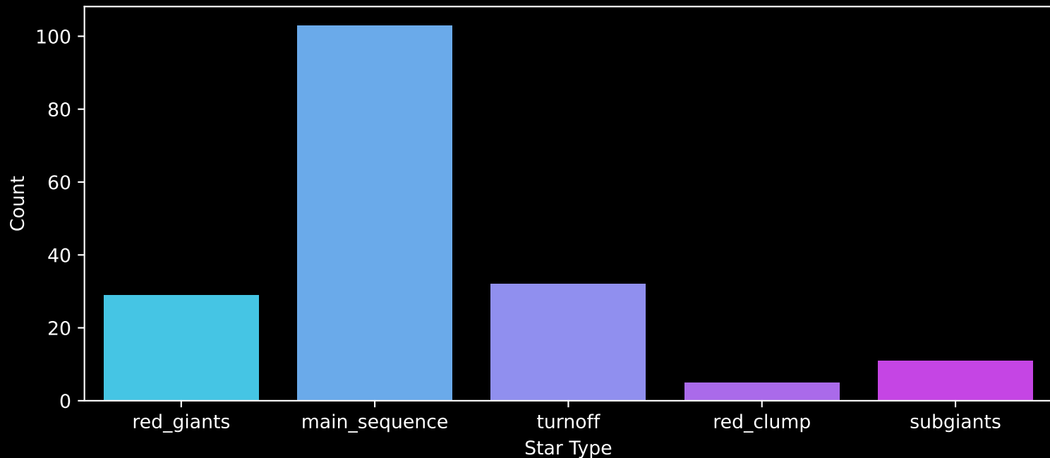
APOGEE DR17 Field: [163+38_MGA] Count plot of Star Type
