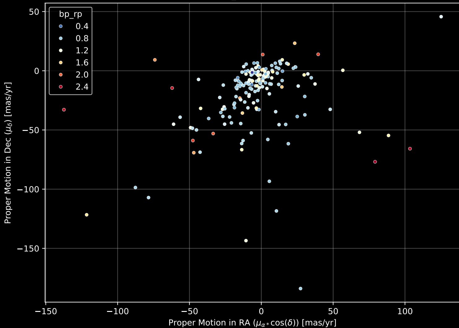
APOGEE DR17 Field: [163+38_MGA] Proper Motion Diagram (n= 180)
