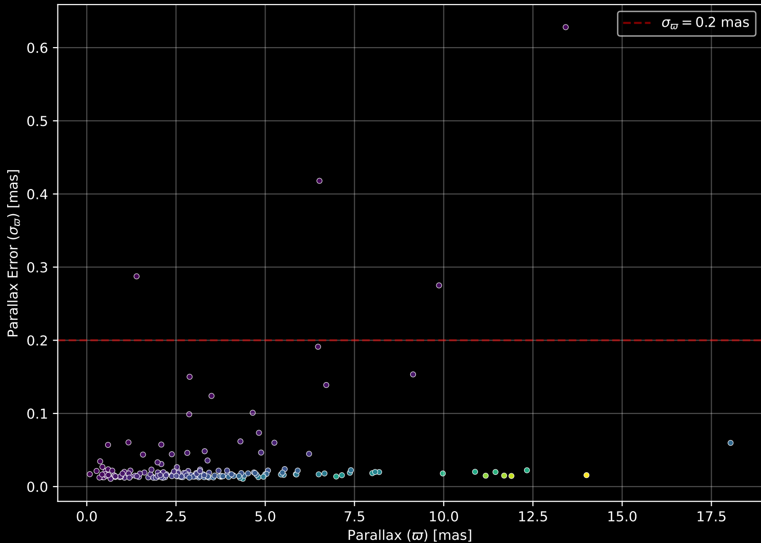
APOGEE DR17 Field: [163+38_MGA] Parallax Quality (n= 180)
